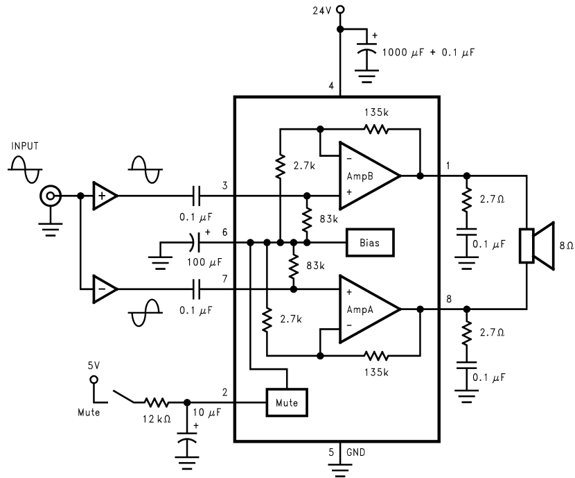
FIGURE 4. Bridge-Mode Application
