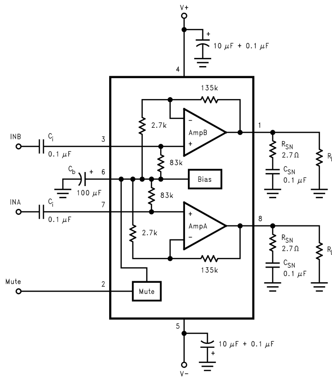
FIGURE 2. Test Circuit
