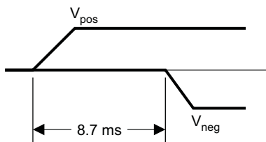
Figure 15. Start-Up Sequencing
