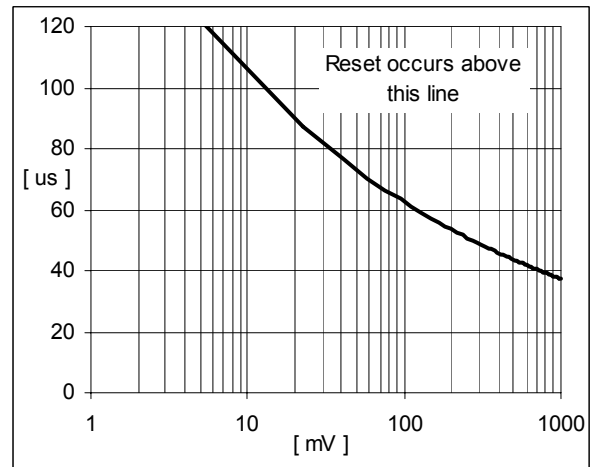
Fig. 11 Maximum Transient Duration t_{\text{SEN}} vs. Overdrive V_{\text{TH}} - V_D
