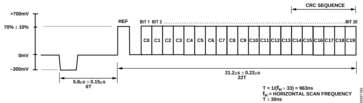
Figure 92. Progressive Scan 525p CGMS Waveform (Line 41)
