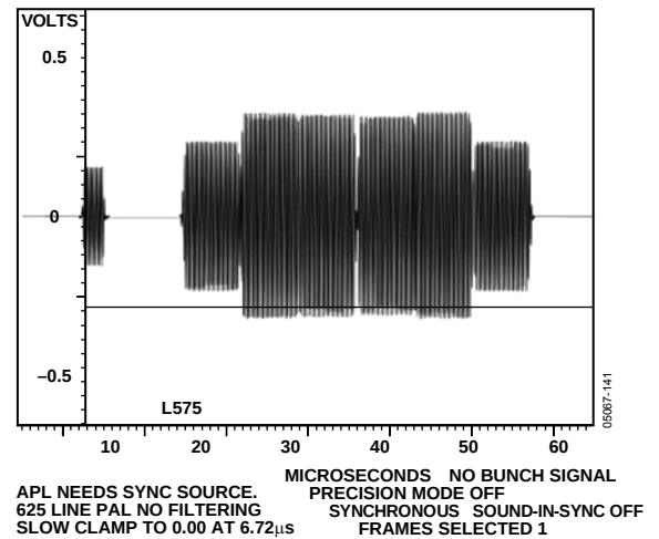
Figure 141. PAL Chroma
