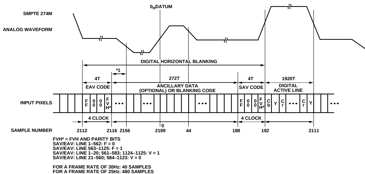
Figure 143. EAV/SAV Input Data Timing Diagram—SMPTE 274M
