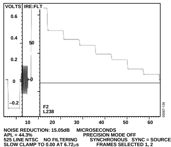
Figure 139. NTSC Luma
