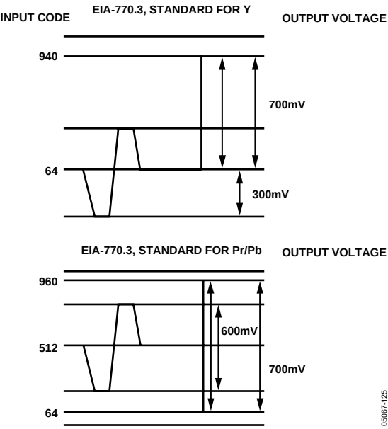
Figure 125. EIA 770.3 Standard Output Signals (1080i/720p)
