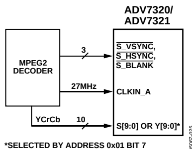
Figure 49. SD Only Input Mode
