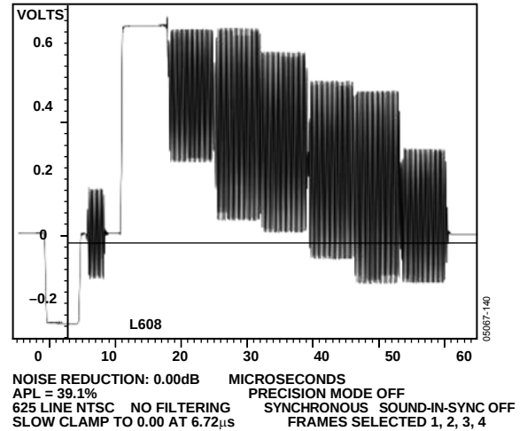
Figure 140. PAL Color Bars 75%
