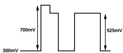
Figure 127. PS RGB Output Levels
