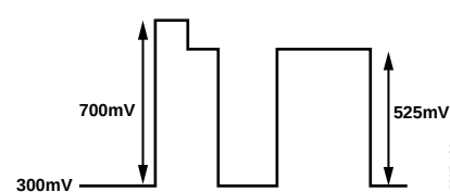
Figure 129. SD RGB Output Levels—RGB Sync Disabled
