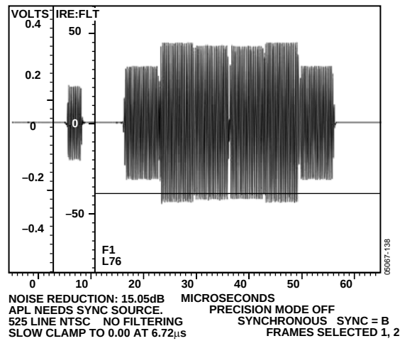
Figure 138. NTSC Chroma
