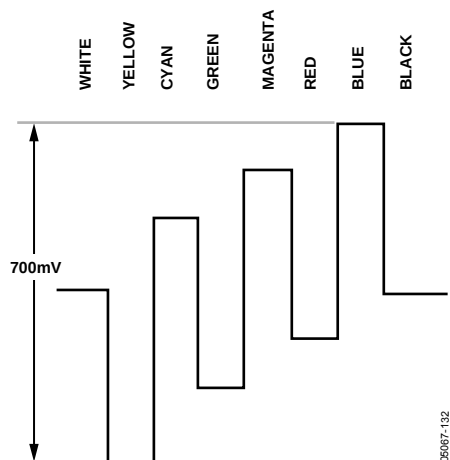
Figure 132. Pb Levels—PAL
