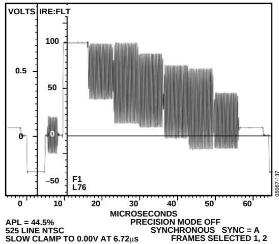
Figure 137. NTSC Color Bars 75%
