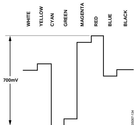
Figure 134. Pr Levels—PAL
