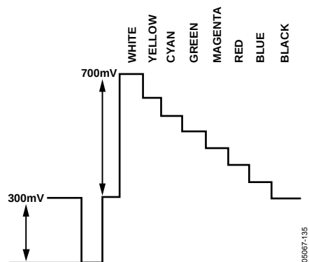
Figure 134. Pr Levels—PAL
