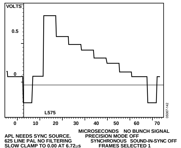
Figure 142. PAL Luma
