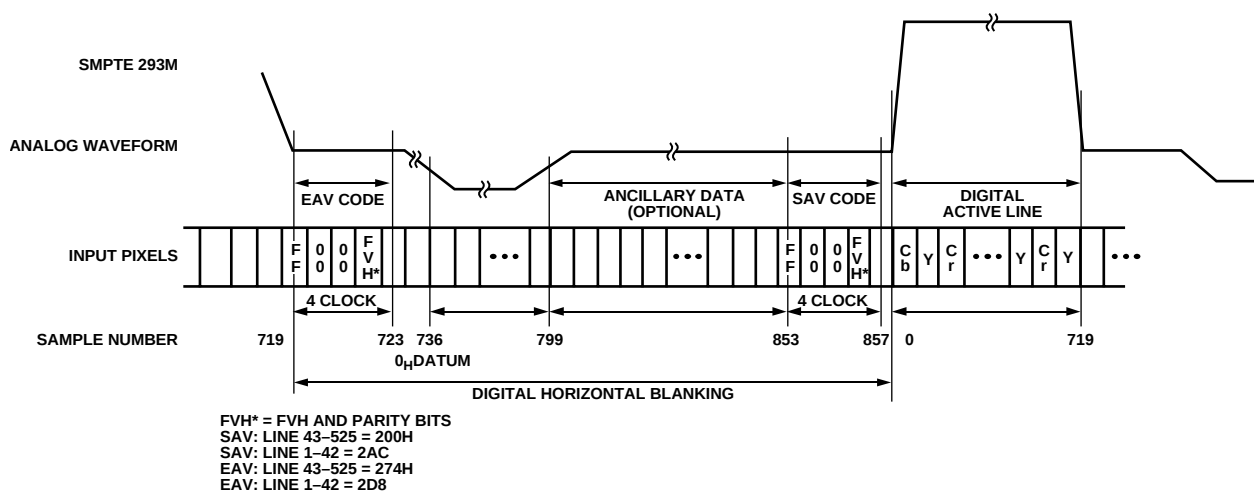
Figure 144. EAV/SAV Input Data Timing Diagram—SMPTE 293M
