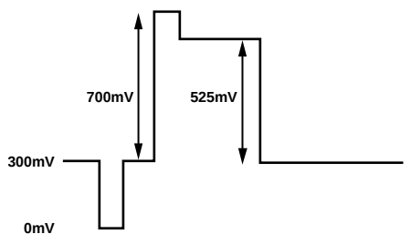
Figure 127. PS RGB Output Levels
