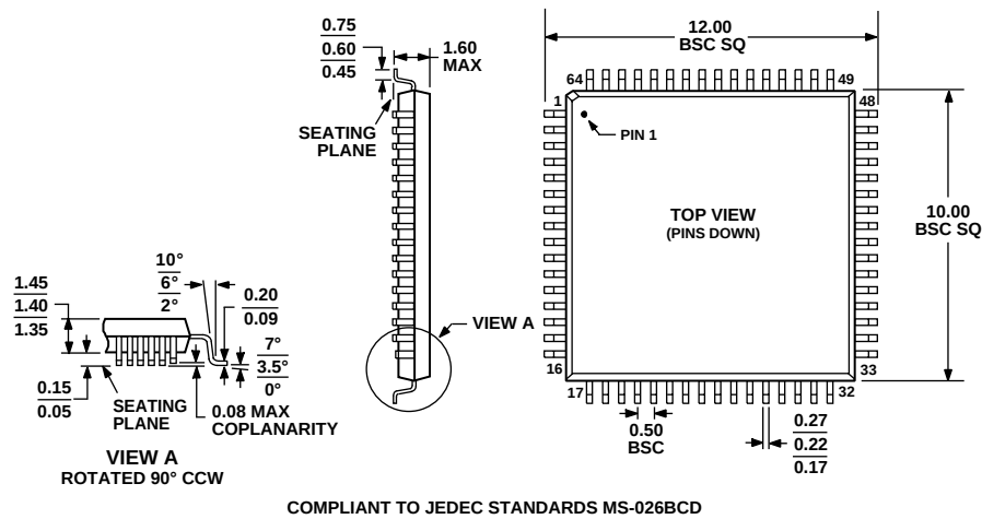
Figure 149. 64-Lead Low Profile Quad Flat Package [LQFP] (ST-64-2) Dimensions shown in millimeters
