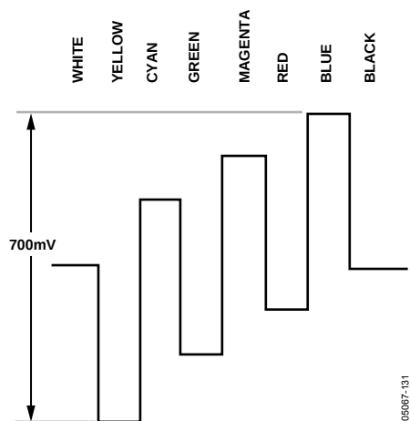
Figure 131. Pb Levels—NTSC
