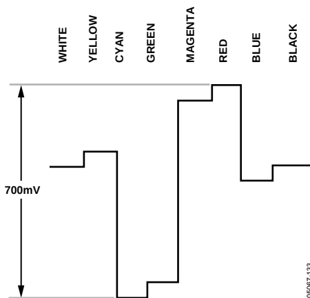
Figure 132. Pb Levels—PAL
