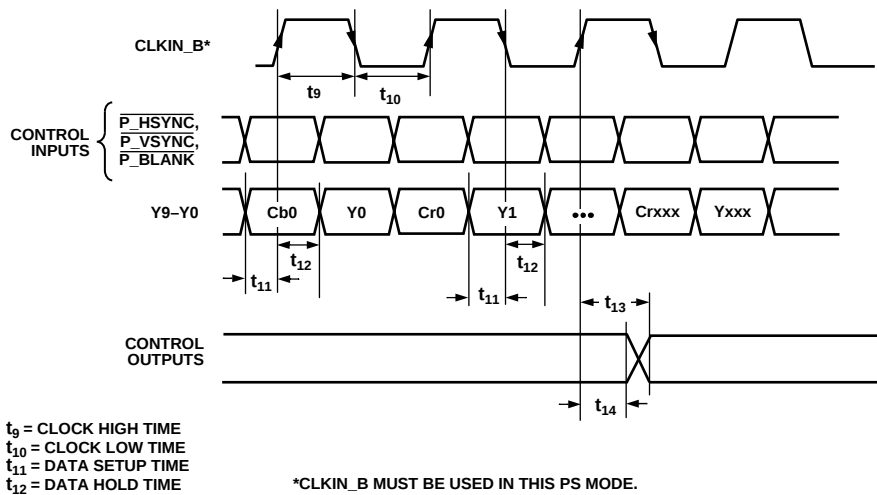
Figure 6. PS 4:2:2 10-Bit Interleaved at 27 MHz \overline{HSYNC}/\overline{VSYNC} Input Mode (Input Mode 100)
