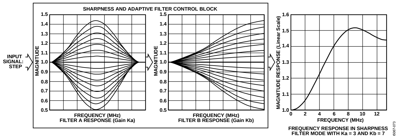
Figure 73. Sharpness and Adaptive Filter Control Block
