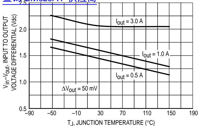
Figure 9. Dropout Voltage
