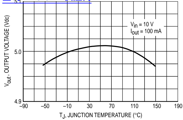
Figure 3. Temperature Stability
