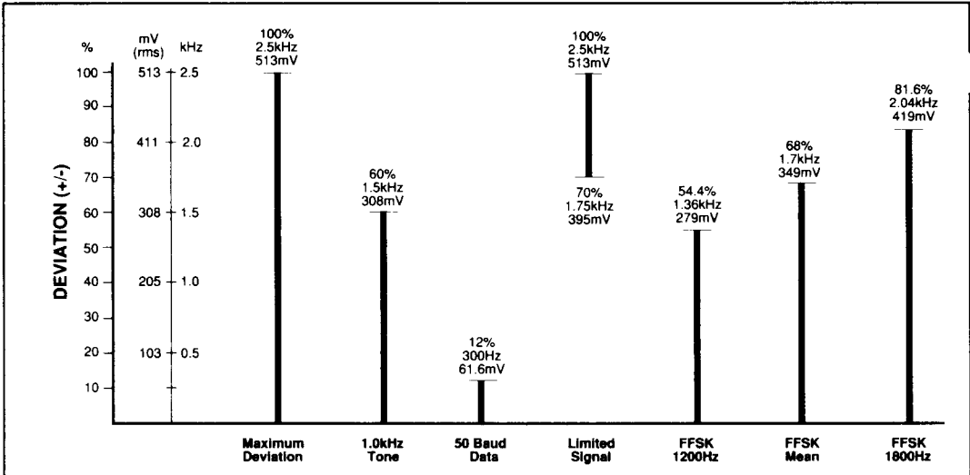
Fig.3 R2000 Signal Deviation Levels and corresponding Tx Mod Outputs with the Mod Level set to 0dB
