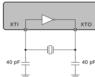
Figure 10. External Component Requirements for Crystal Circuit
