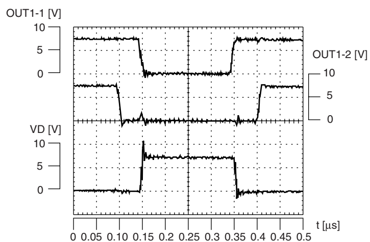
Switching waveform
