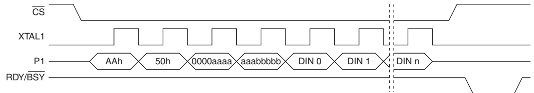
Figure 22-10. Write Code Page Sequence
