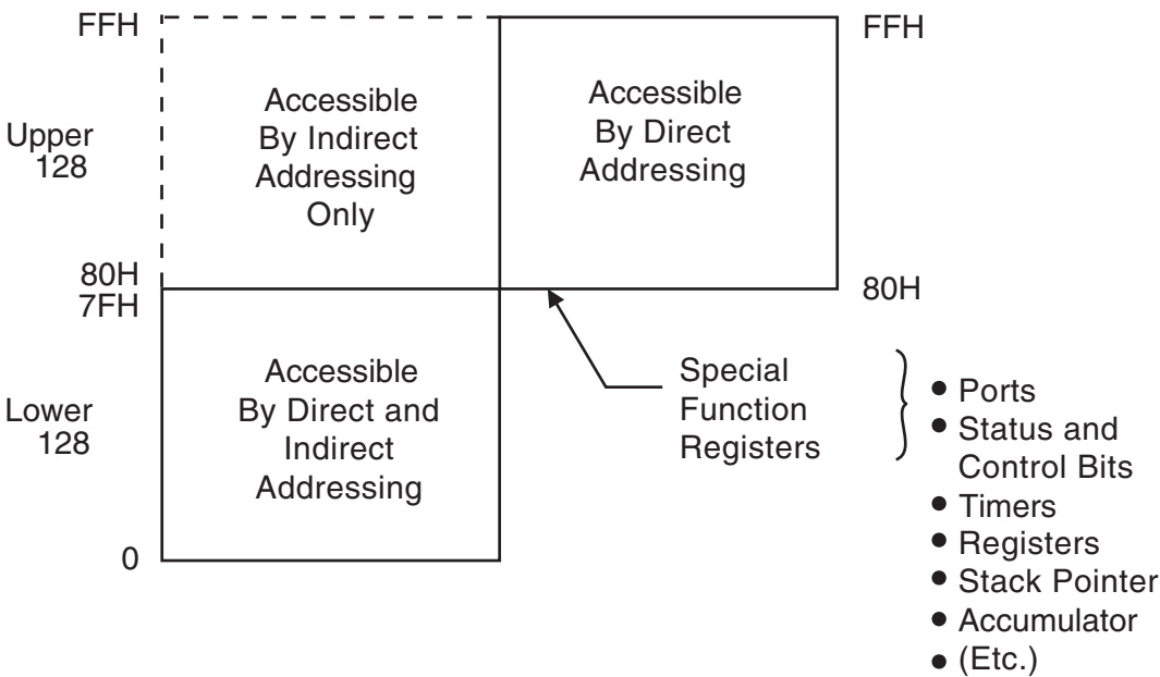
Figure 5-2. Data Memory Map
