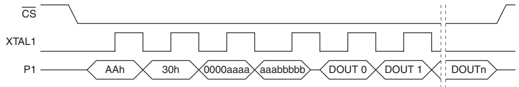
Figure 22-11. Read Code Page Sequence
