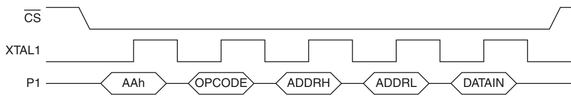
Figure 22-3. Parallel Write Command Sequence
