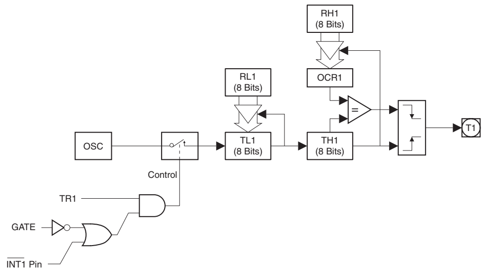
Figure 15-7. Timer/Counter 1 PWM Mode 1
