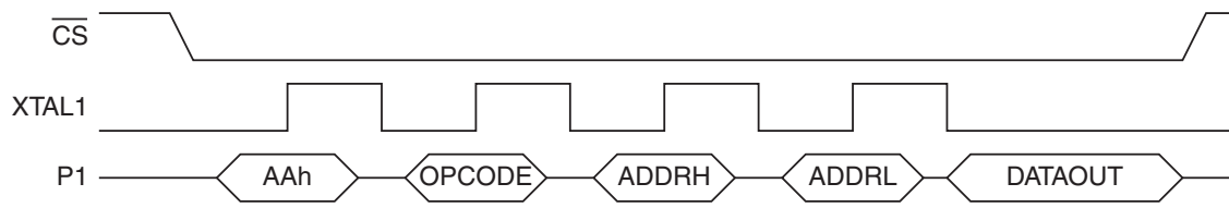
Figure 22-4. Parallel Read Command Sequence
