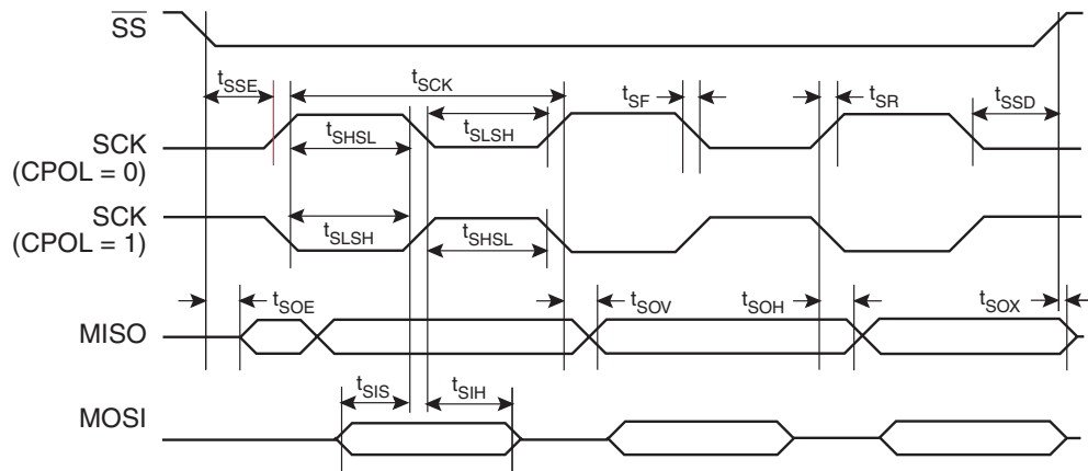
Figure 23-4. SPT Slave Timing (CPHA = 1)
