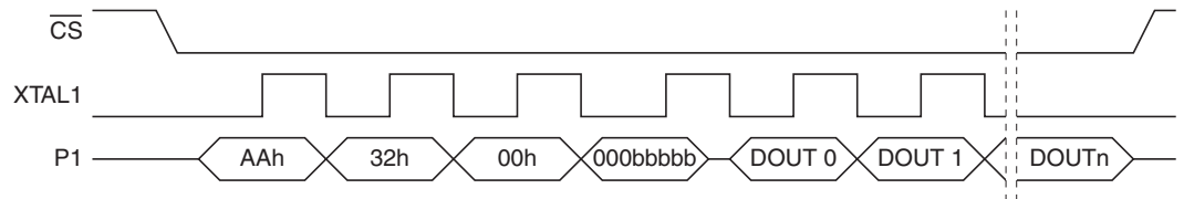
Figure 22-13. Read User Signature Page Sequence
