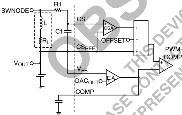
Figure 11. Lossless Inductive Current Sensing with Enhanced V^2
