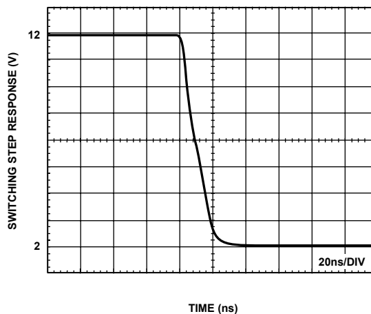
Figure 16. Invert Switching Step Response (Falling Edge), 10 V Step, C_L = 200 pF
