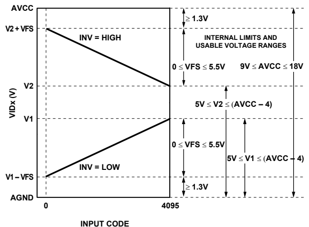
Figure 36. Transfer Function and Usable Voltage Ranges
