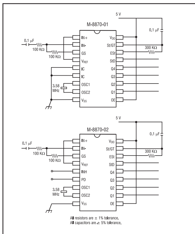
Figure 4 Single-Ended Input Configuration
