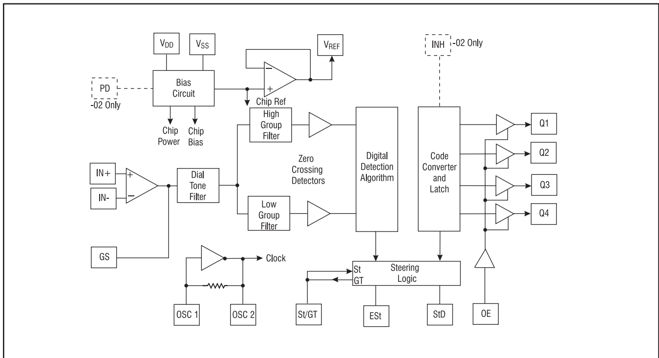
Figure 2 Block Diagram
