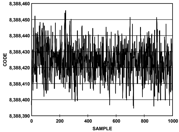
Figure 10. Noise ( V_{REF} = AV_{DD} , Update Rate = 10 Hz, Gain = 128)
