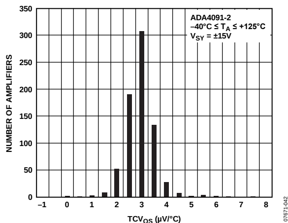
Figure 30. TCVOS Distribution
