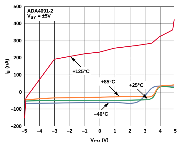
Figure 21. Input Bias Current vs. Common-Mode Voltage
