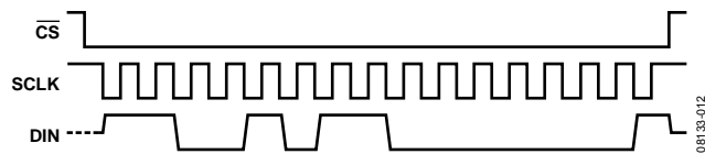
Figure 16. SPI Sequence for a Wake-Up Command (DIN = 0xCB01)
