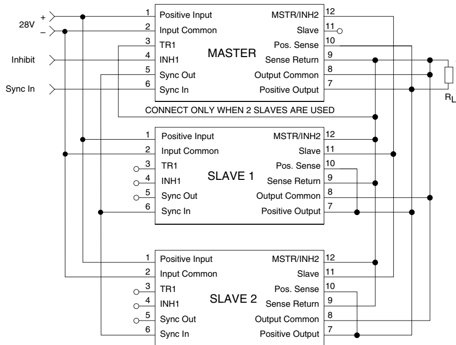
FIGURE 2: PARALLEL CONNECTIONS
