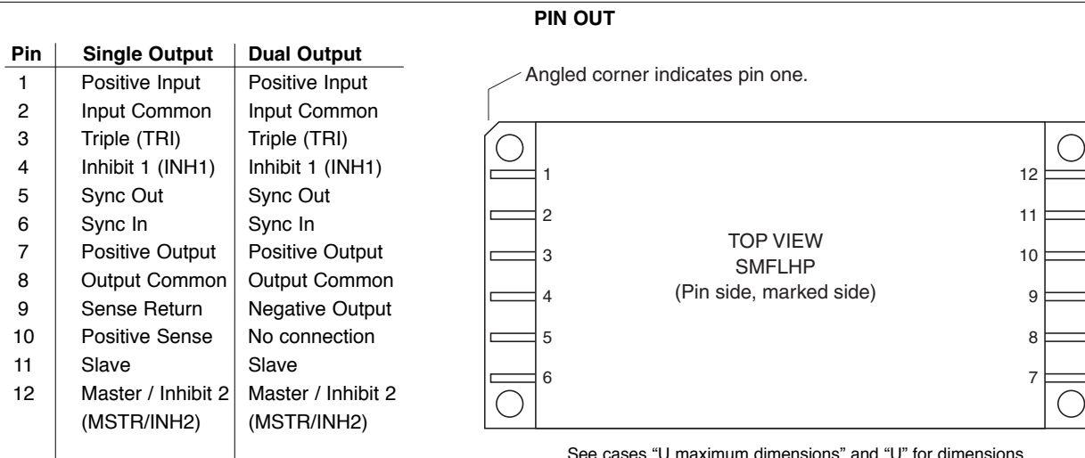
FIGURE 3: PIN OUT
