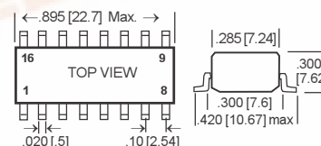
Type EC3AG & EC3HG (16-pin SMD *)
