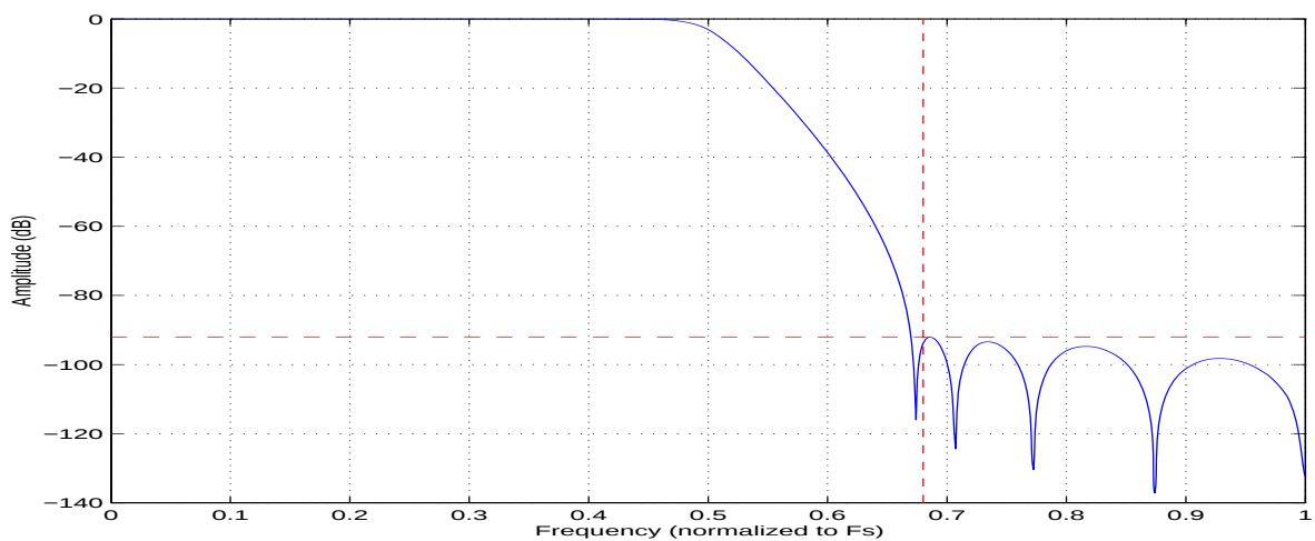
Figure 23. DSM Stopband
