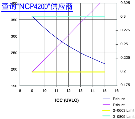
Figure 10. Typical Shunt Resistor Value and Power Dissipation for Different UVLO Voltage
