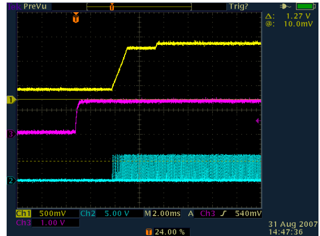
Figure 9. Overcurrent Latchoff Waveforms
