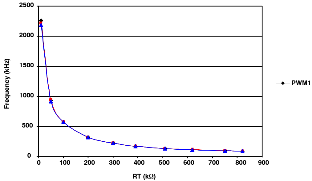
Figure 3. Master Clock Frequency vs. RT
