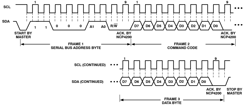
Figure 12. Write Byte
