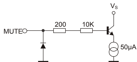
PINS: MUTE
