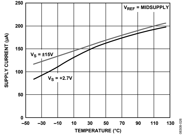
Figure 28. Supply Current per Channel vs. Temperature
