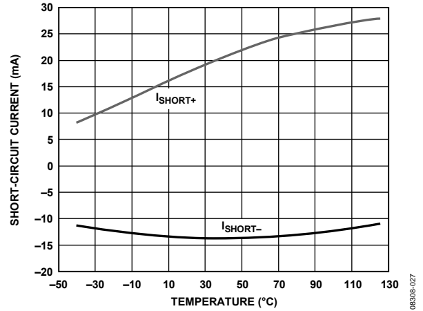
Figure 29. Short-Circuit Current per Channel vs. Temperature
