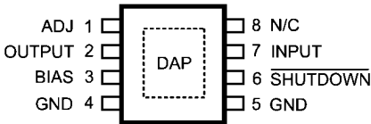
PSOP-8, Top View
