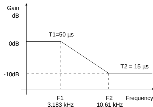
Figure 11. De-Emphasis Curve
