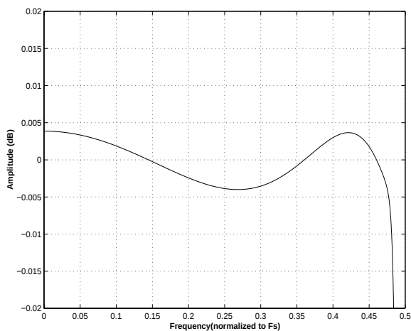
Figure 16. Single-Speed (fast) Passband Ripple
