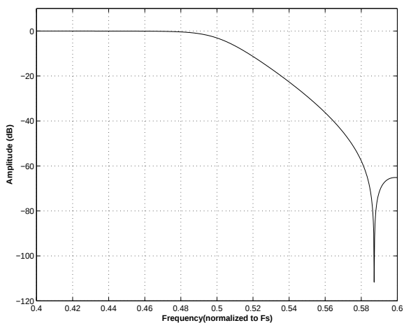
Figure 18. Single-Speed (slow) Transition Band
