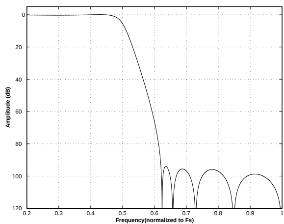
Figure 29. Quad-Speed (fast) Stopband Rejection
