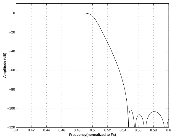
Figure 14. Single-Speed (fast) Transition Band
