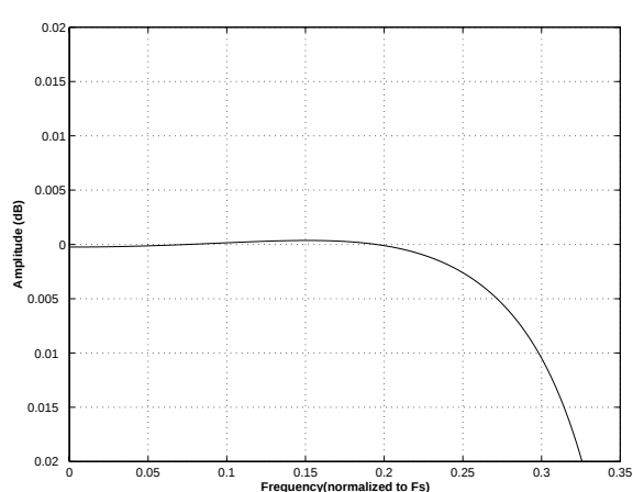
Figure 28. Double-Speed (slow) Passband Ripple
