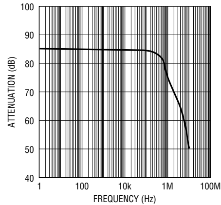
Reference Feedthrough
