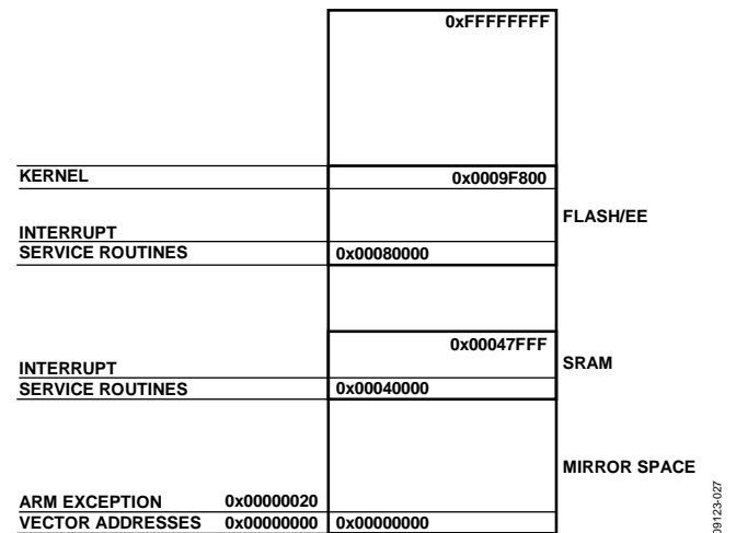
Figure 39. Remap for Exception Execution
