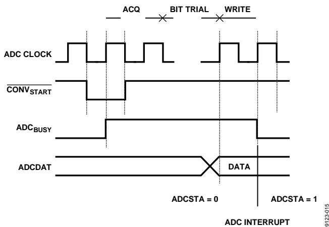
Figure 30. ADC Timing
