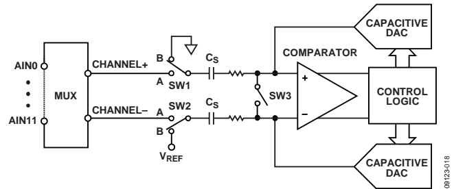
Figure 32. ADC Conversion Phase
