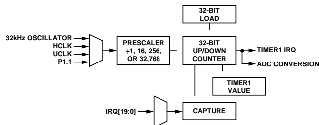
Figure 53. Timer1 Block Diagram
