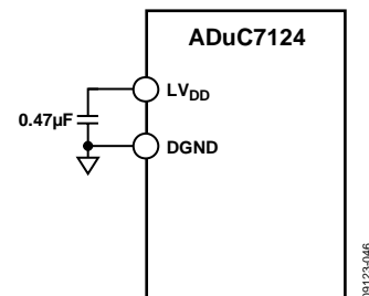
Figure 59. Voltage Regulator Connections
