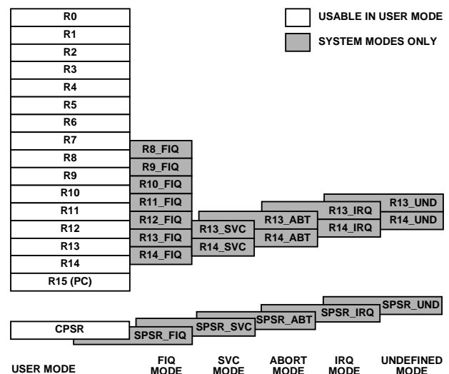
Figure 22. Register Organization
