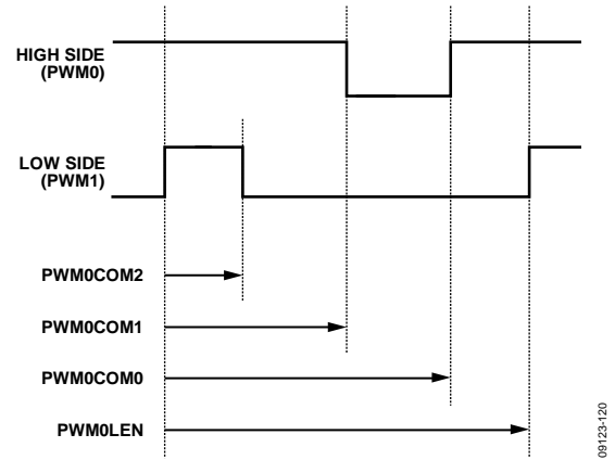
Figure 48. PWM Timing
