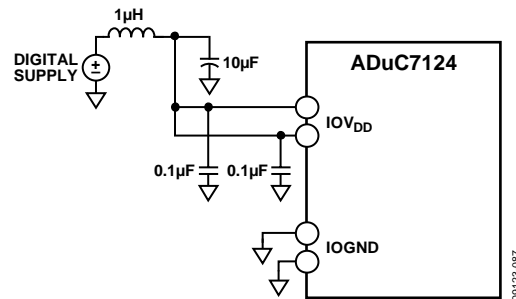
Figure 58. Recommended IOV_{DD} Supply Filter
