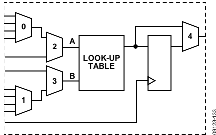
Figure 50. PLA Element
