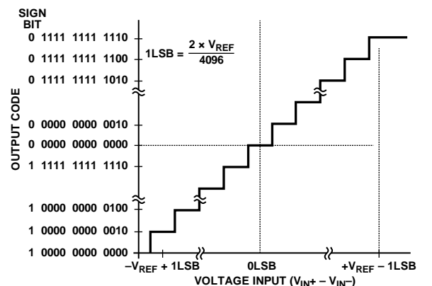
Figure 28. ADC Transfer Function in Differential Mode
