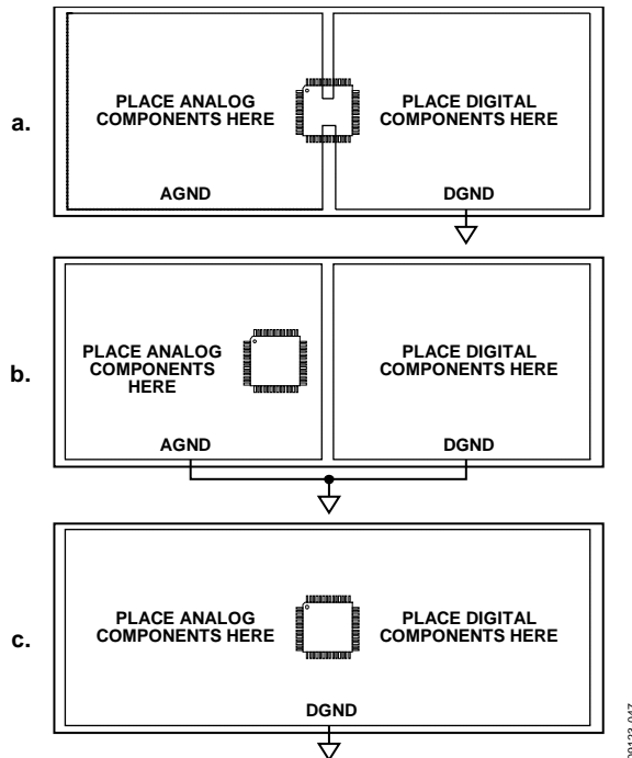
Figure 60. System Grounding Schemes
