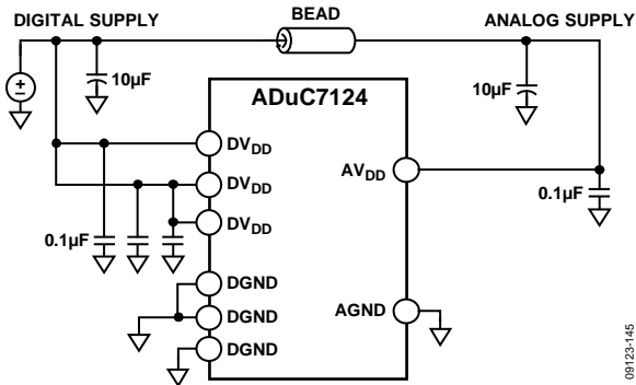
Figure 57. External Single Supply Connections
