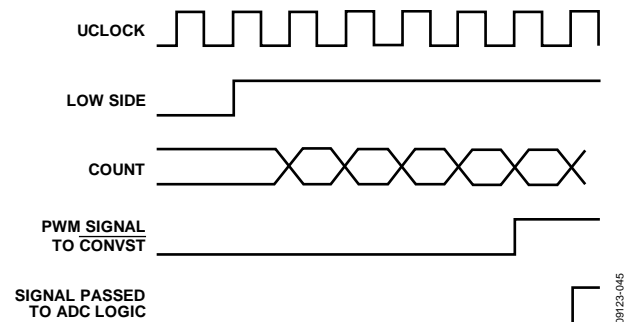
Figure 49. ADC Conversion
