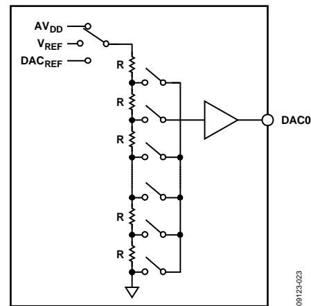
Figure 40. DAC Structure
