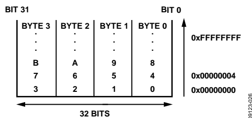
Figure 24. Little Endian Format
