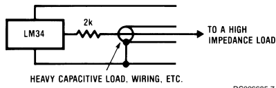
FIGURE 3. LM34 with Decoupling from Capacitive Load
