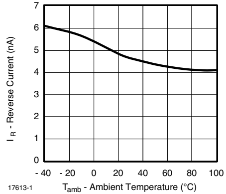
Figure 5. Reverse Current vs. Ambient Temperature
