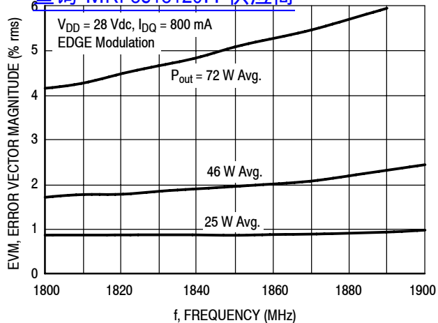
Figure 6. EVM versus Frequency
