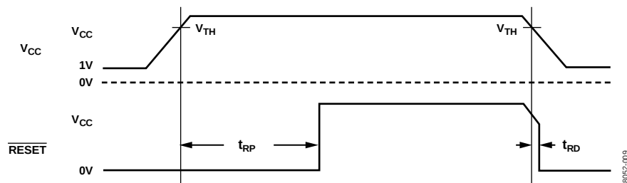
Figure 9. \overline{\text{RESET}} Timing
