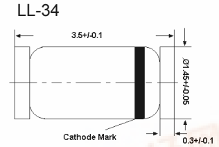
Glass case MiniMELF Dimensions in mm
