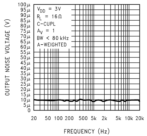
Noise Floor
