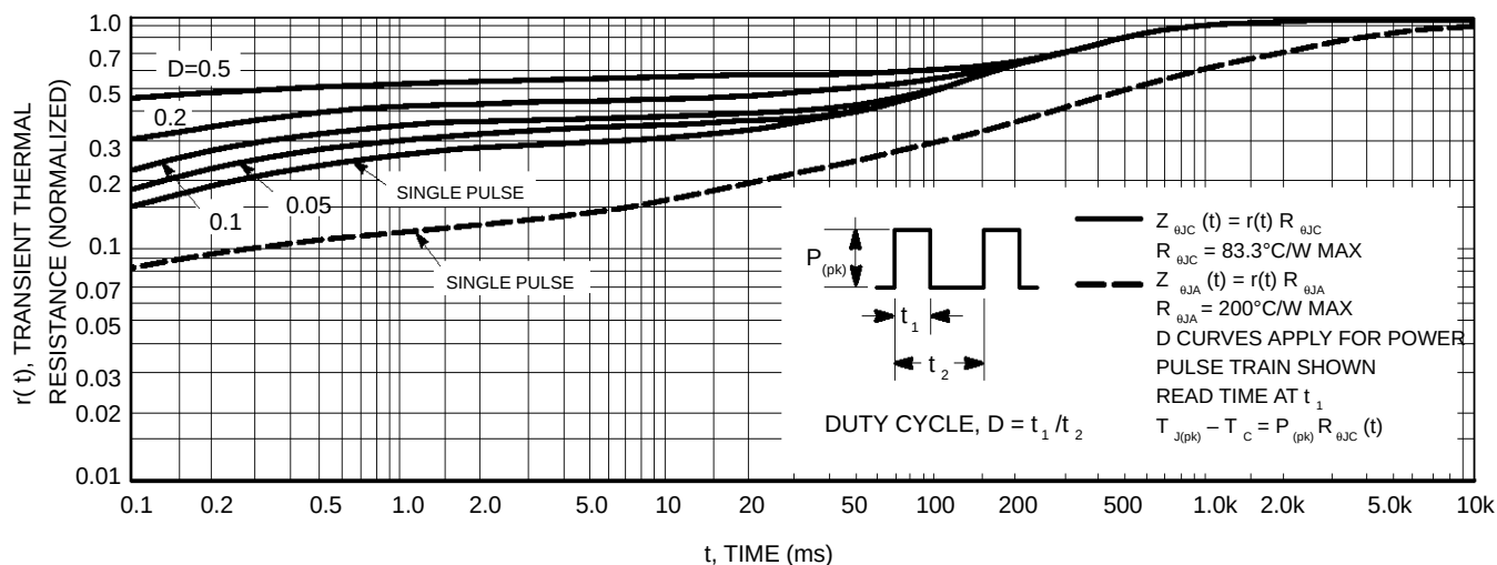
Figure 13. Thermal Response
