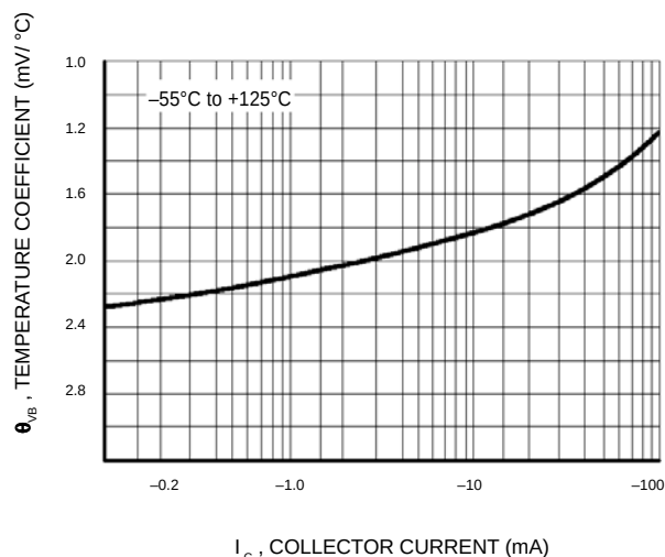
Figure 4. Base-Emitter Temperature Coefficient
