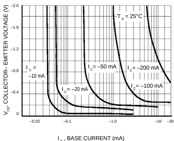
Figure 3. Collector Saturation Region
