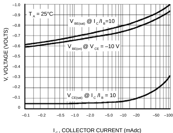
Figure 2. "Saturation" and "On" Voltages
