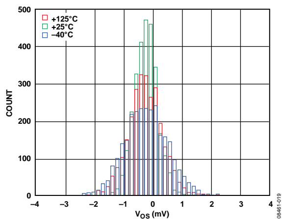
Figure 20. Offset Distribution
