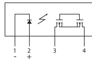
CPC1973Y Pinout
