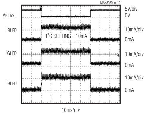
RGB—PLAY_ON/OFF TRANSITION, LOGIC-LOW
