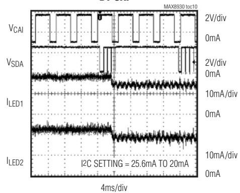
WLED—DIMMING CURRENT TRANSIENT BY CAI
