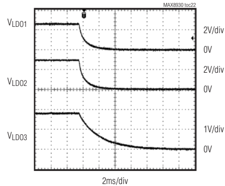
LDO SHUTDOWN—DEFAULT ACTIVE DISCHARGE ON
