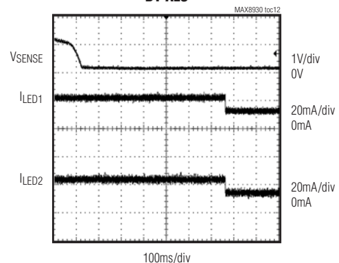
WLED—DIMMING CURRENT TRANSIENT BY ALC
