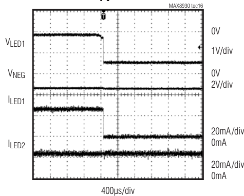
WLED—LED1 OPEN CIRCUIT, V_{PV} = 3.2V
