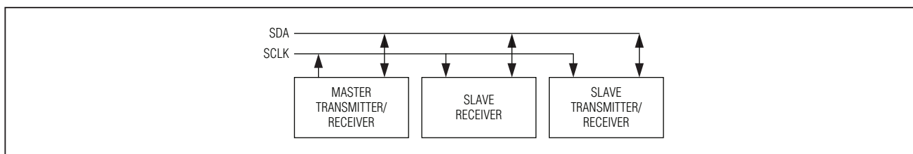
Figure 12. I 2 C Master and Slave Configuration
