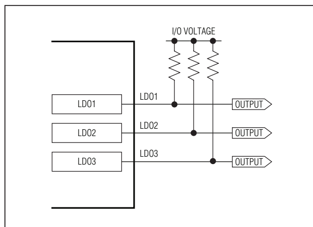
Figure 9. LDO GPO Configuration
