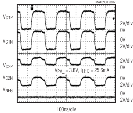
WLED—CHARGE PUMP ACTIVE
