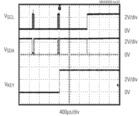
KEY—ON/OFF BY I2C
