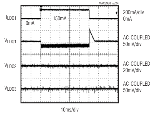
LD01 LOAD TRANSIENT
