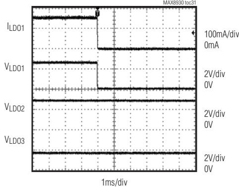
LD01 SHORT CIRCUIT
