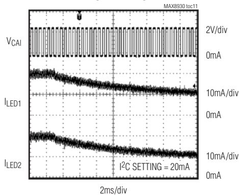
WLED—DIMMING CURRENT TRANSIENT BY CAI AND I 2 C
