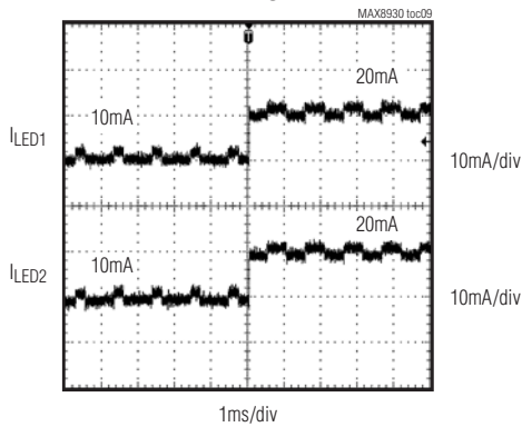
WLED—DIMMING CURRENT TRANSIENT BY I 2 C
