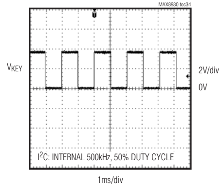
KEY—ON/OFF BY INTERNAL PWM, NO SLOPE
