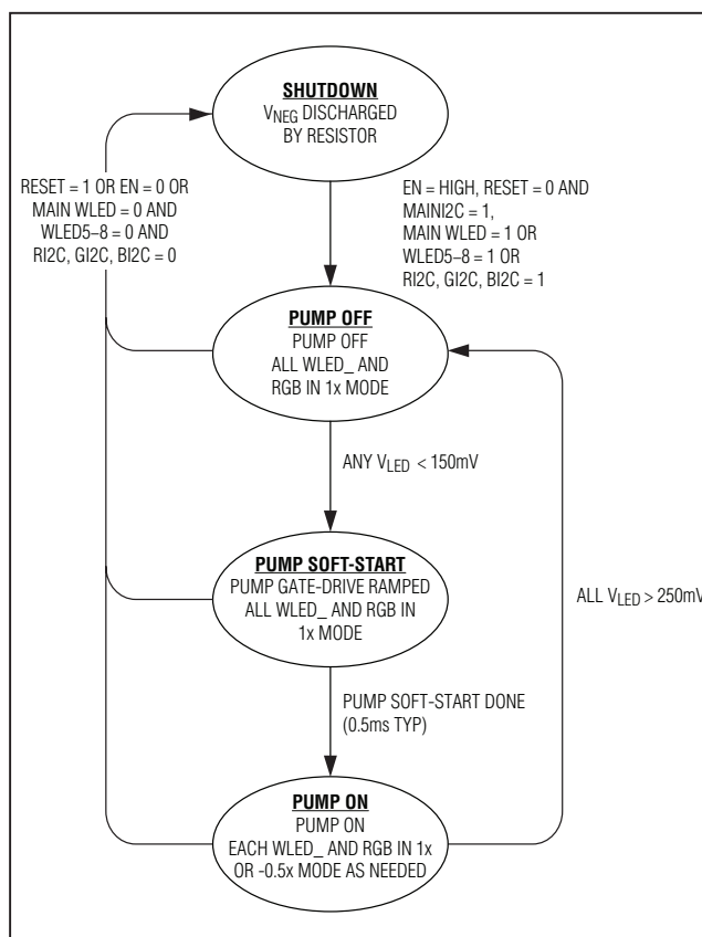
Figure 2. Startup and Mode Change Algorithm
