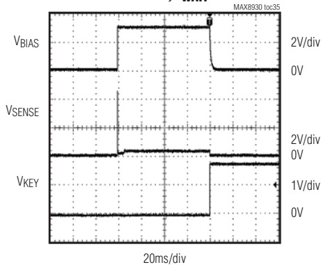
ALC—STARTUP, t WAIT = 64ms
