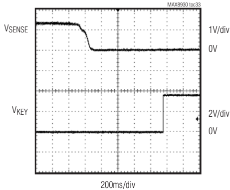
KEY—ON/OFF BY ALC
