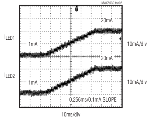
WLED—DIMMING CURRENT TRANSIENT WITH SLOPE CONTROL
