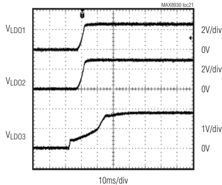
LDO STARTUP—NO LOAD
