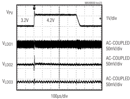
LDO—LINE TRANSIENT
