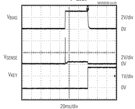
ALC—STARTUP, t WAIT = 32ms
