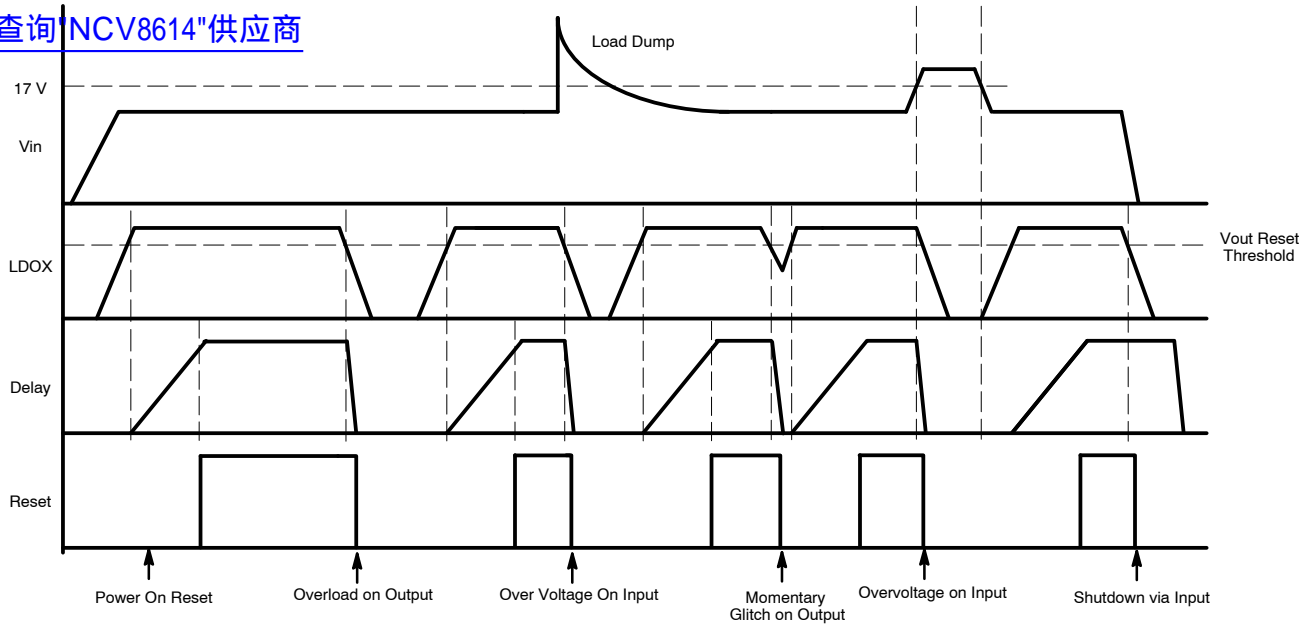
Figure 5. NCV8614 Reset Timing Diagram
