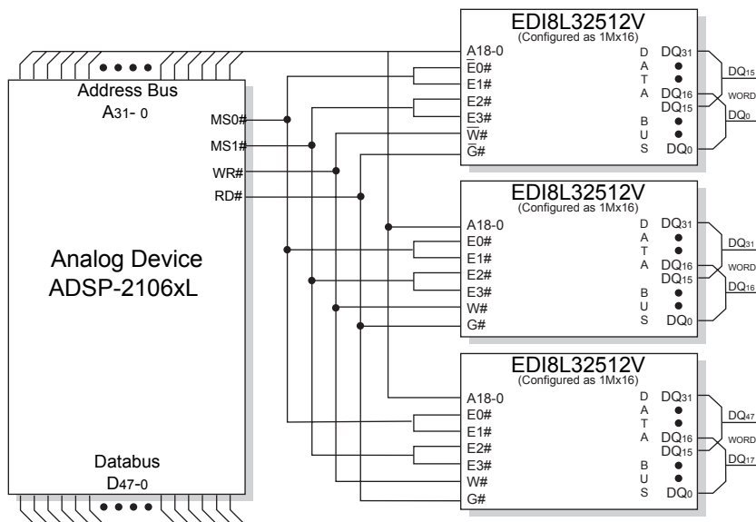
INTERFACING THE ANALOG SHARC DSP WITH THE EDI8L32512V (1M X 48 ARRAY)
