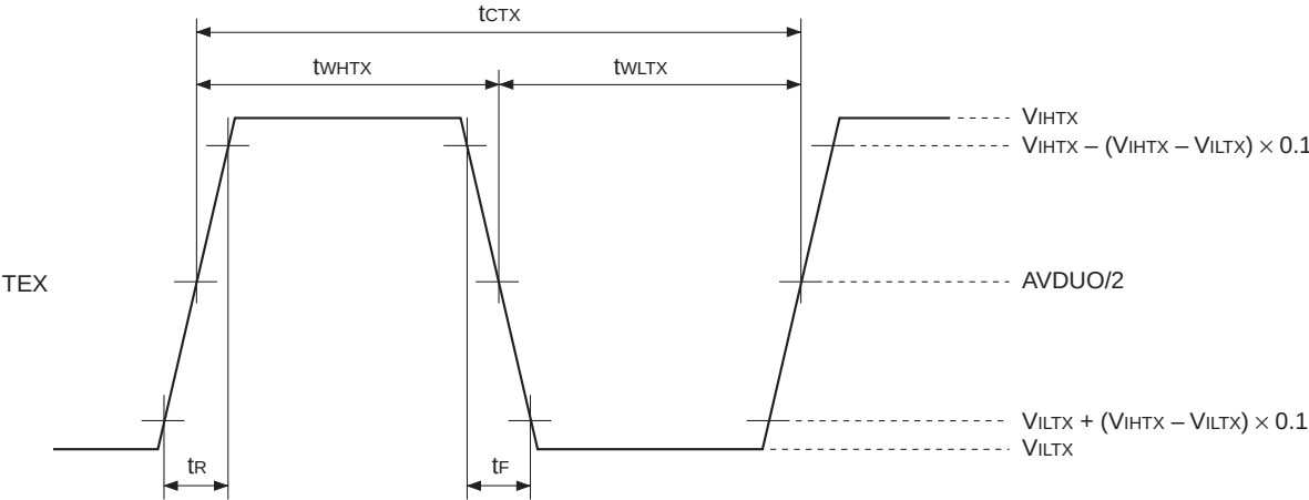
Fig. 2. Sub Clock Timing
