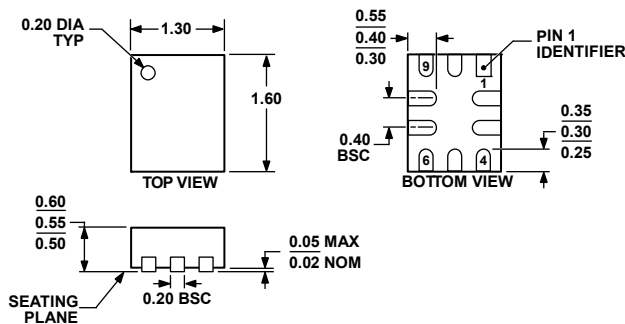
COMPLIANT TO JEDEC STANDARDS MS-012-AA Figure 68. 10-Lead Lead Frame Chip Scale Package [LFCSP_UQ] 1.30 mm x 1.60 mm, Body, Ultra Thin Quad (CP-10-10) Dimensions shown in millimeters
