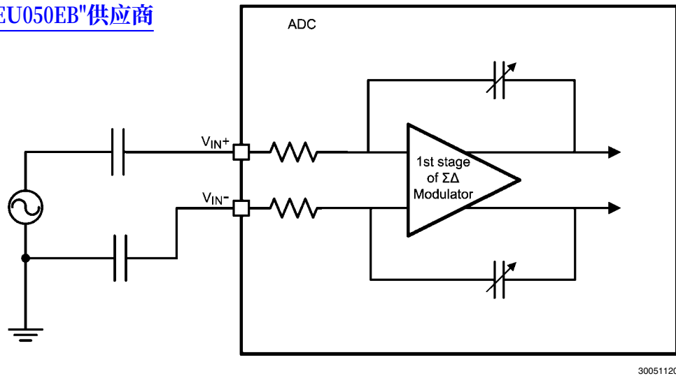
FIGURE 14. Single Ended Input
