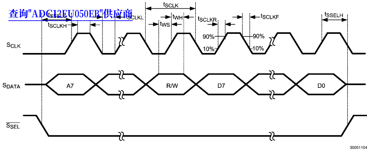
FIGURE 3. SPI Write Timing
