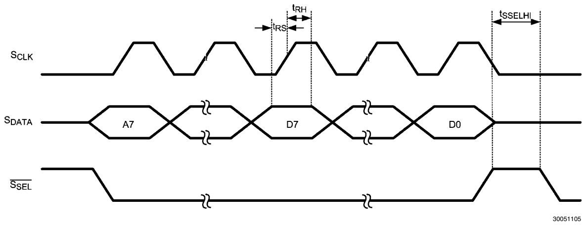
FIGURE 4. SPI Read Timing
