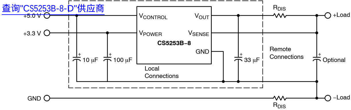
Figure 16. Remote Sense
