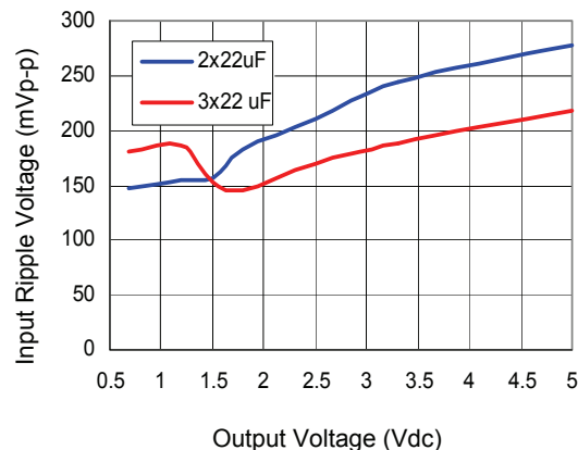
Figure 40. Input ripple voltage for various output voltages with 2x22 μF or 3x22 μF ceramic capacitors at the input (20A load). Input voltage is 12V.
