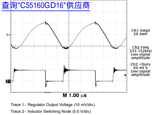
Figure 8. CS5160 Peak-to-Peak Ripple on V_{OUT} = 2.8\text{ V} , I_{OUT} = 13\text{ A} (Heavy Load)
