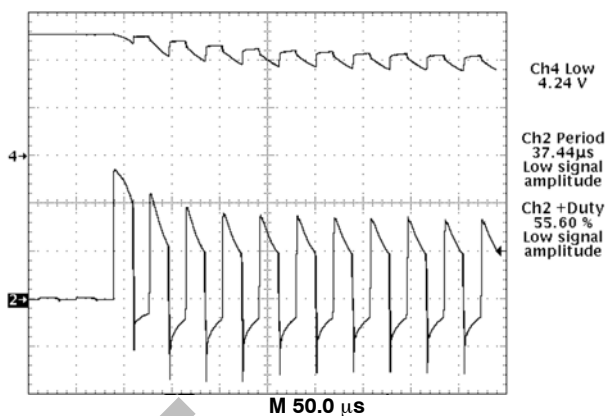
Figure 13. CS5160 Startup with Regulator Output Shorted
