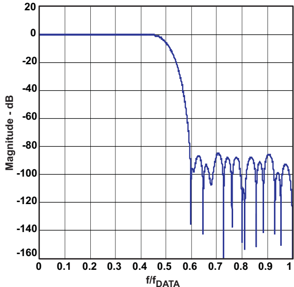
Figure 39. 2x Interpolation Composite Response
