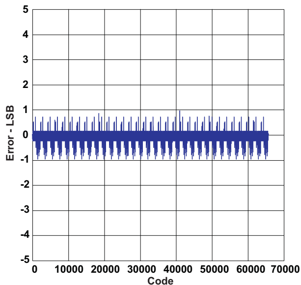
Figure 2. DIFFERENTIAL NON-LINEARITY
