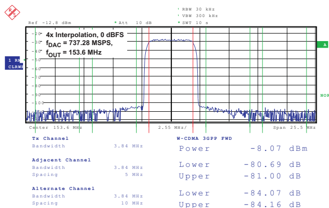
Figure 22. SINGLE CARRIER W-CDMA TEST MODEL 1
