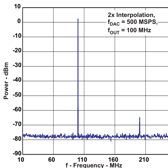
Figure 10. SINGLE TONE SPECTRAL PLOT
