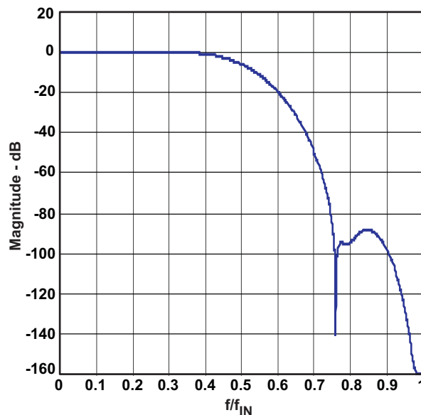
Figure 38. Magnitude Spectrum for FIR1
