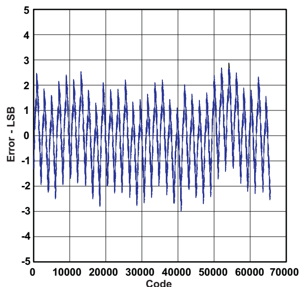
Figure 1. INTEGRAL NON-LINEARITY
