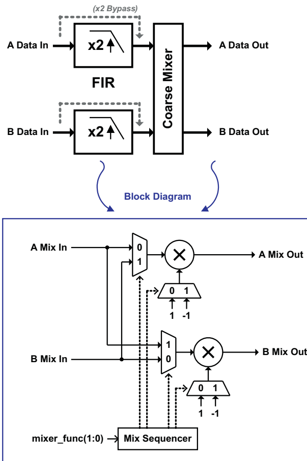
Figure 41. Coarse Mixers Block Diagram
