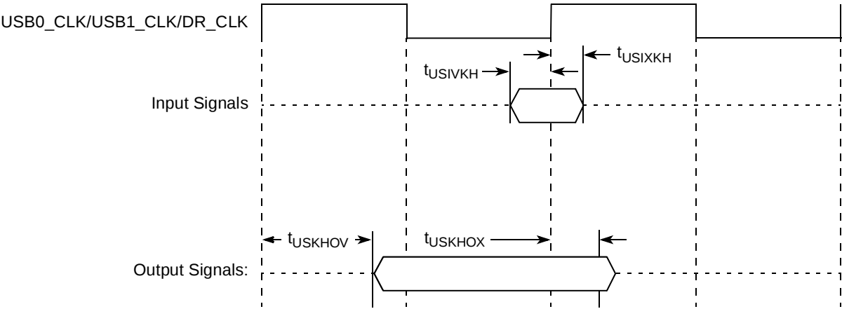
Figure 17. USB Signals
