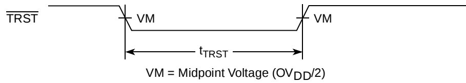
Figure 27. \overline{TRST} Timing Diagram
