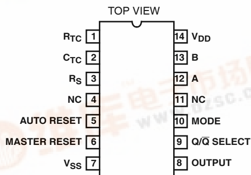
CD4541B (CERDIP, PDIP, SOIC, SOP, TSSOP)
