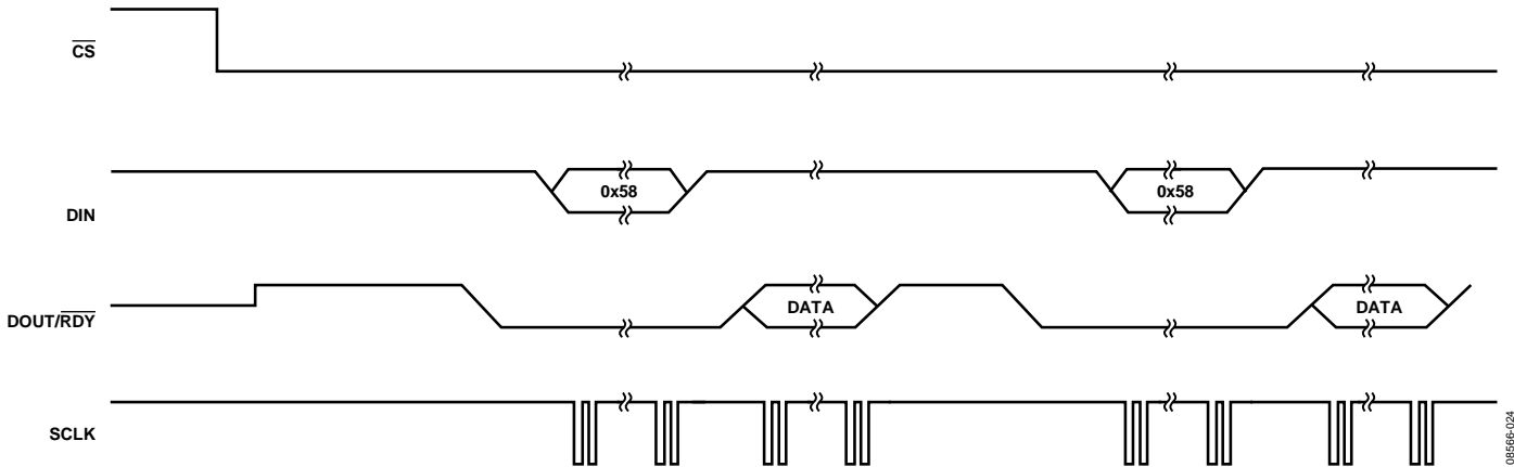
Figure 25. Continuous Conversion
