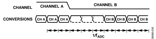
Figure 36. Sinc 3 Channel Change
