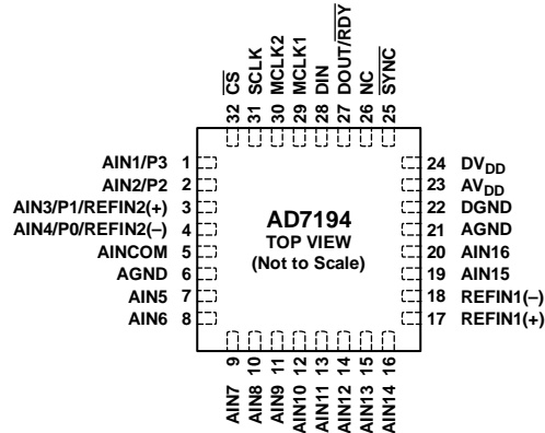
Figure 5. Pin Configuration
