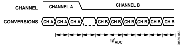
Figure 54. Fast Settling, Sinc 4 Filter
