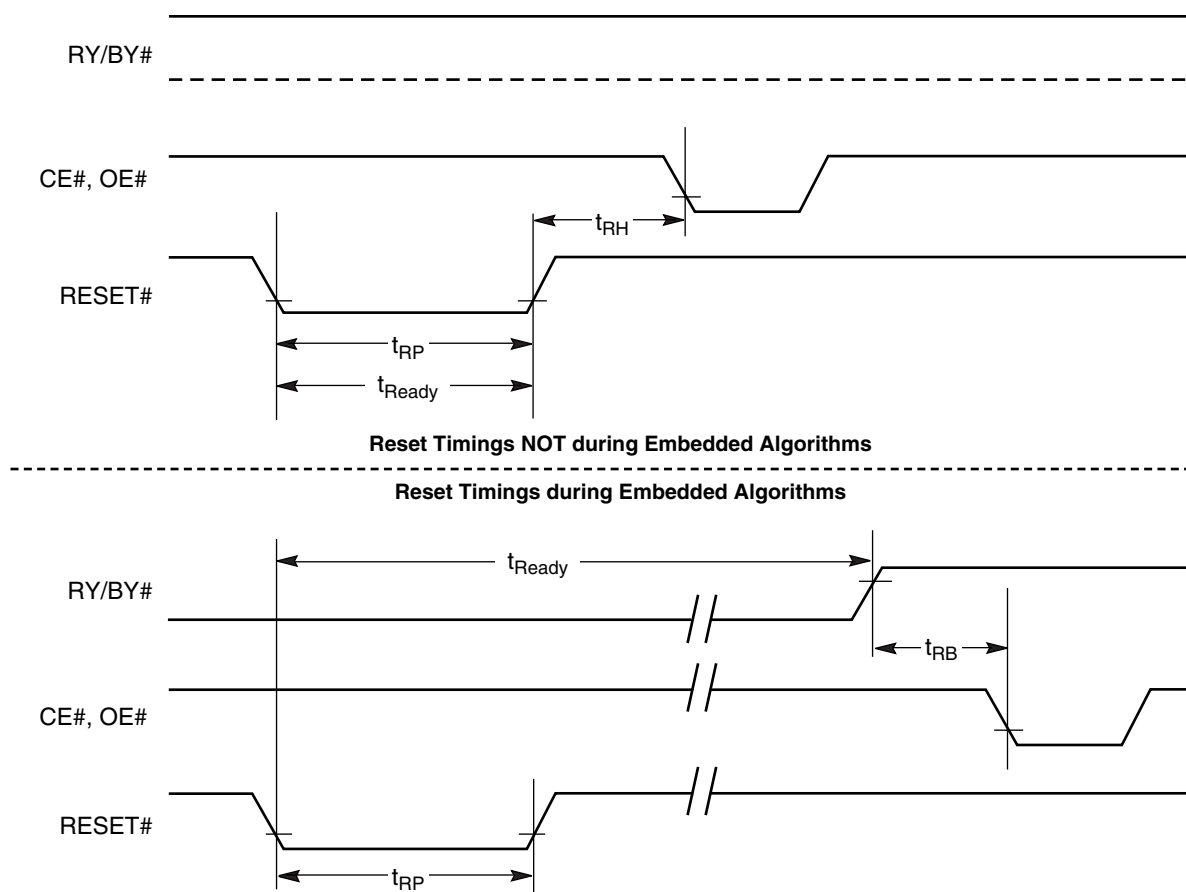
Figure 14. RESET# Timings
