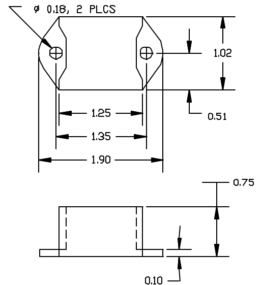
E Package
