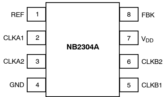
Figure 2. Pin Configuration
