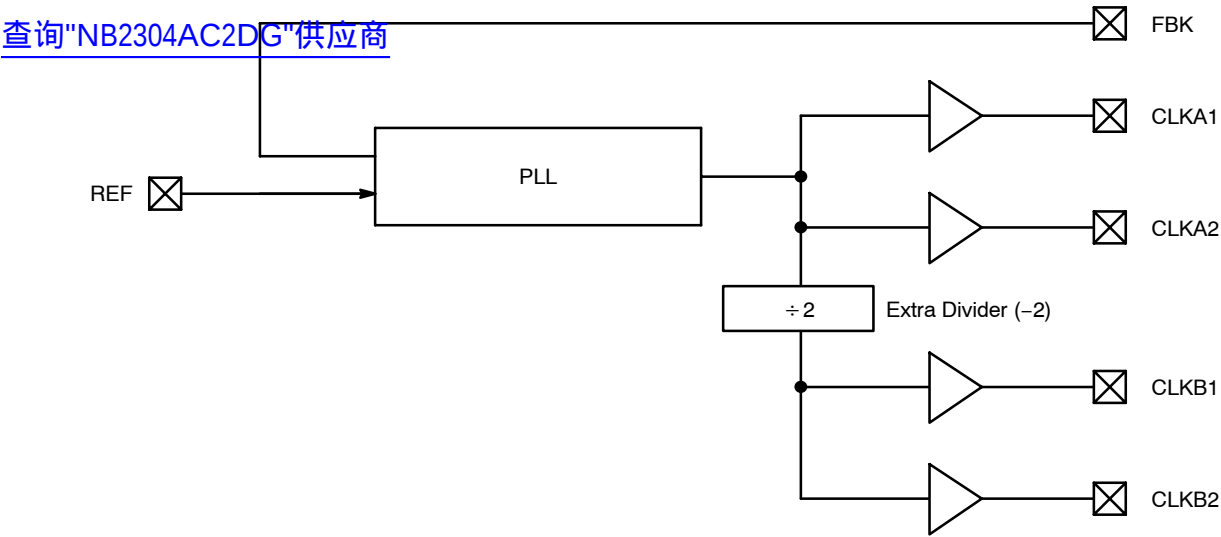
Figure 1. Basic Block Diagram (see Figures 11 and 12 for device specific Block Diagrams)
